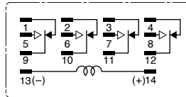
4PDT (RY4/RM42)
